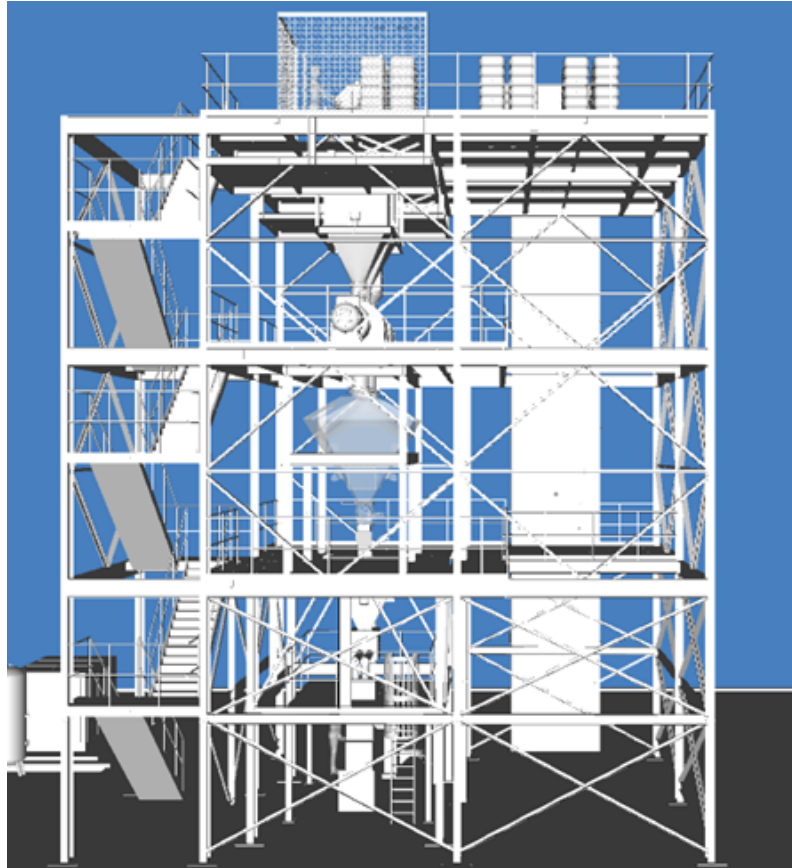
3D Model of Batching Plant Structure
