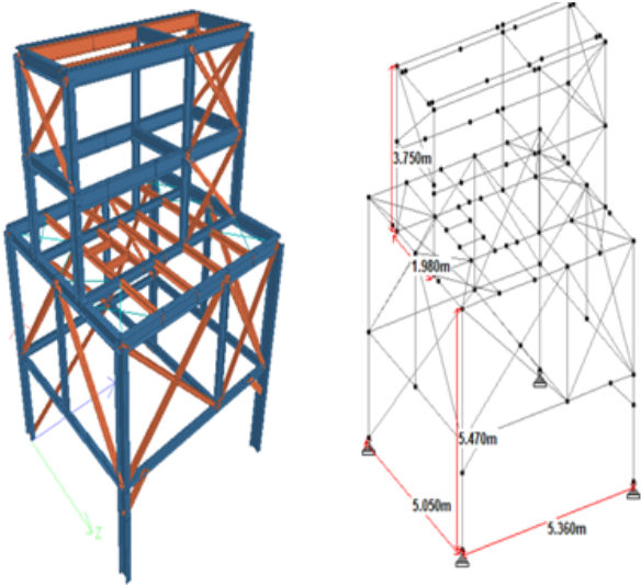
Mixes Structure – Staad Geometry
